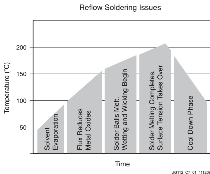
Figure 7-1: Soldering Sequence
